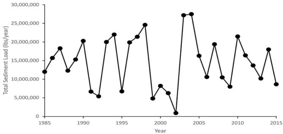
Figure 17. Long-term changes in A. Total nitrogen, B. Total phosphorus, and C. Total sediments above the fall-line in the Mattaponi River from 1984 through 2015. Data shown are estimates (without flow normalization) provided by the US Geological Survey's River Input Monitoring program.
