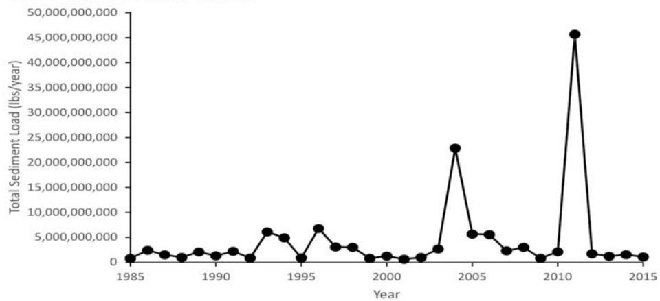
Figure 29. Long-term changes in A. Total nitrogen, B. Total phosphorus, and C. Total sediment loads at the fall-line in the Susquehanna River from 1985 through 2015. Data shown are log-transformed estimates (without flow normalization) provided by the US Geological Survey's River Input Monitoring program.
