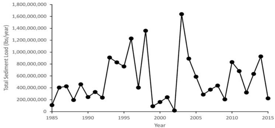
Figure 23. Long-term changes in A. Total nitrogen, B. Total phosphorous, and C. Total sediment loads at the fall-line in the Rappahannock River from 1985 through 2015. Data shown are estimates (without flow normalization) provided by the US Geological Survey's River Input Monitoring program.
